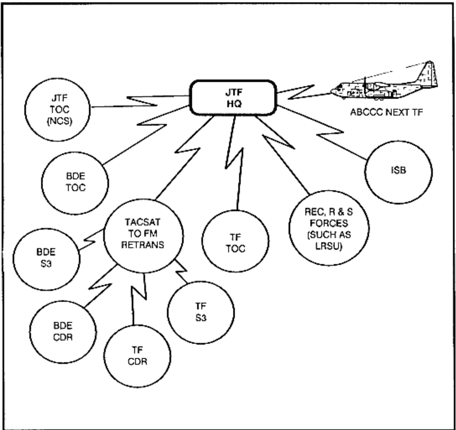
Figure 10-14. JTF TACSAT VHF voice net.
